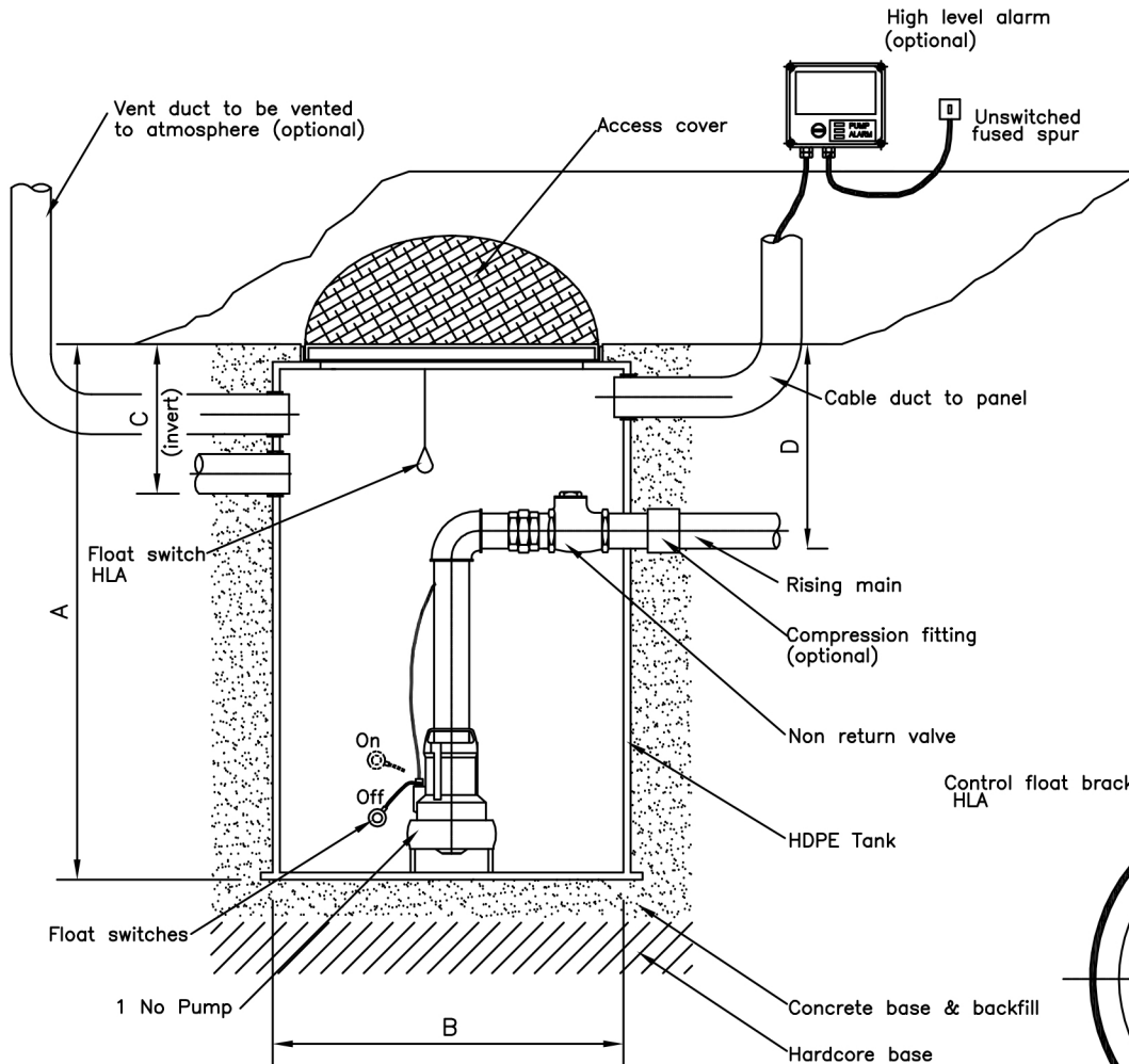
SIDE ELEVATION
